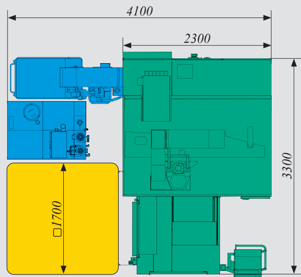
Example with high-pressure internal cooling and pallet changer. Green: machine Blue: periphery/coolant equipment / Yellow: automation
