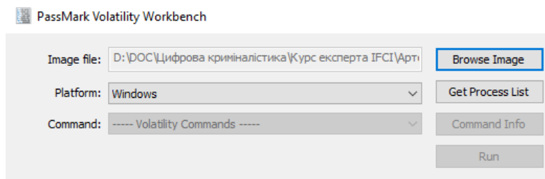
Рис. 87. Volatility Workbench
