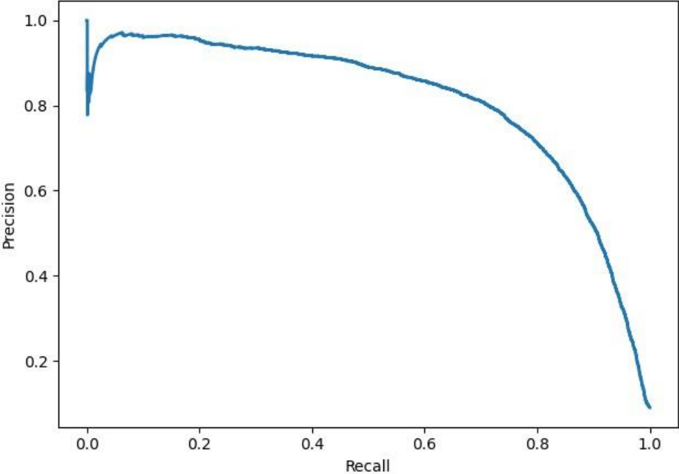
Precision-Recall curve
